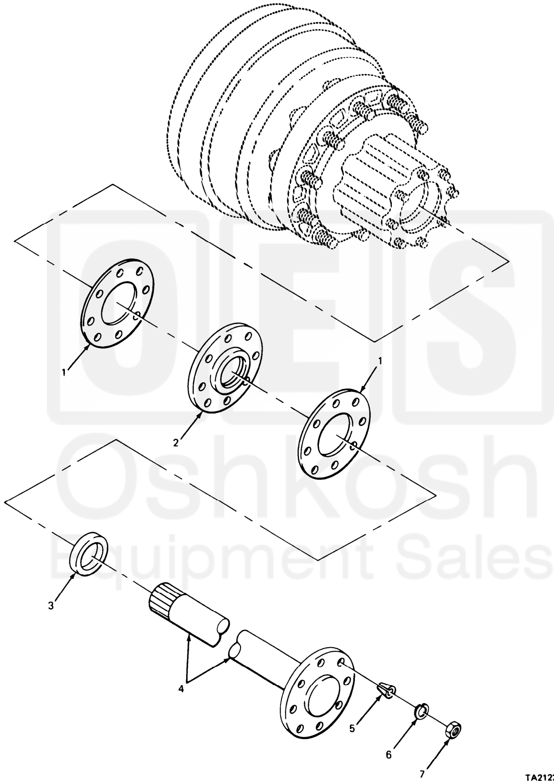
FIGURE 151. AXLE SHAFT AND RELATED PARTS.
